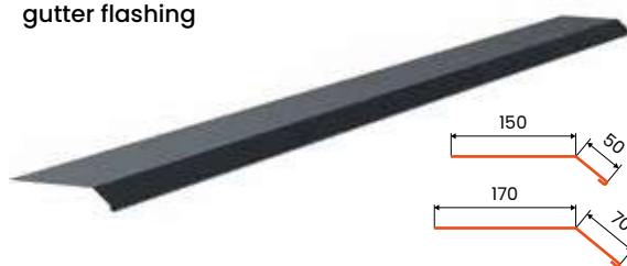
gutter flashing
