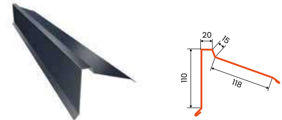
PHR mono-pitched roof termination
