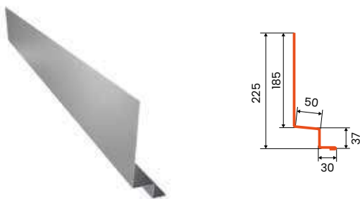
PHR side joining flashing
