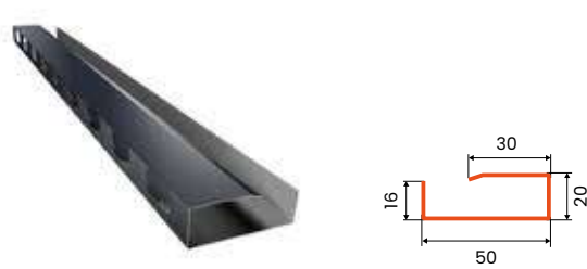
PHR ridge tile flashing
