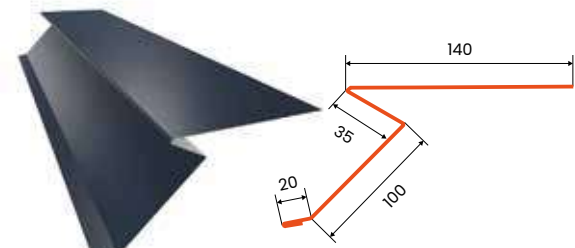
PHR large troughed gutter flashing
