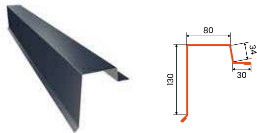
PHR wind brace
