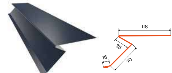
PHR troughed gutter flashing
