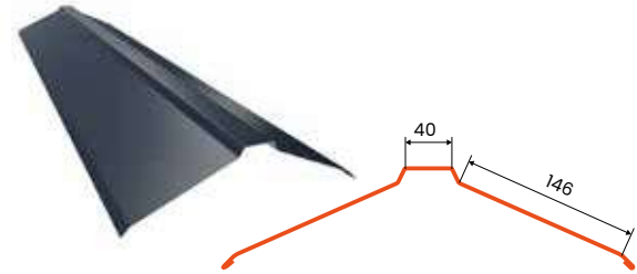
PHR troughed ridge tile
