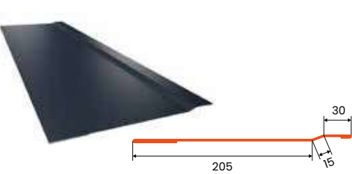
PHR joining flashing
